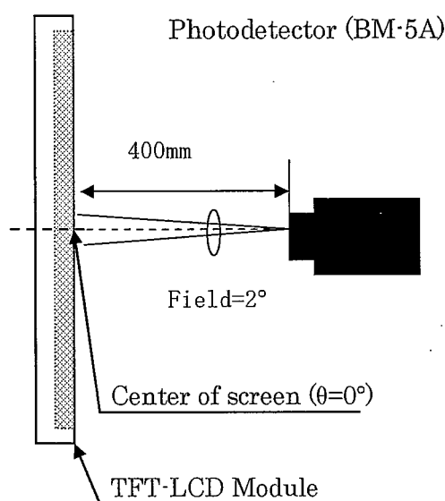
Fig.3-2 Measurement Method ( • Luminance • Contrast ratio • Chromaticity )
