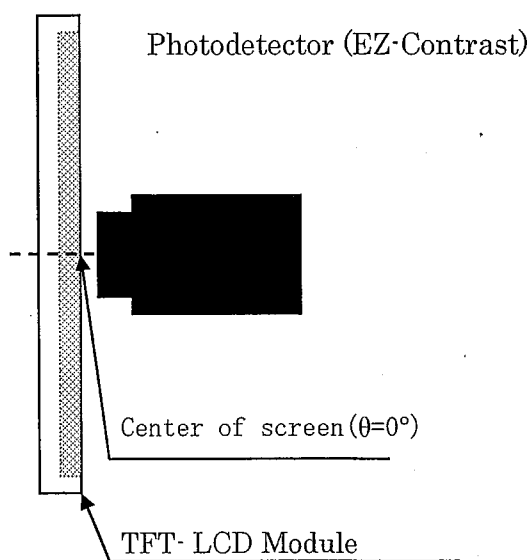
Fig.3-1 Measurement Method ( • Viewing angle range • Response time )
