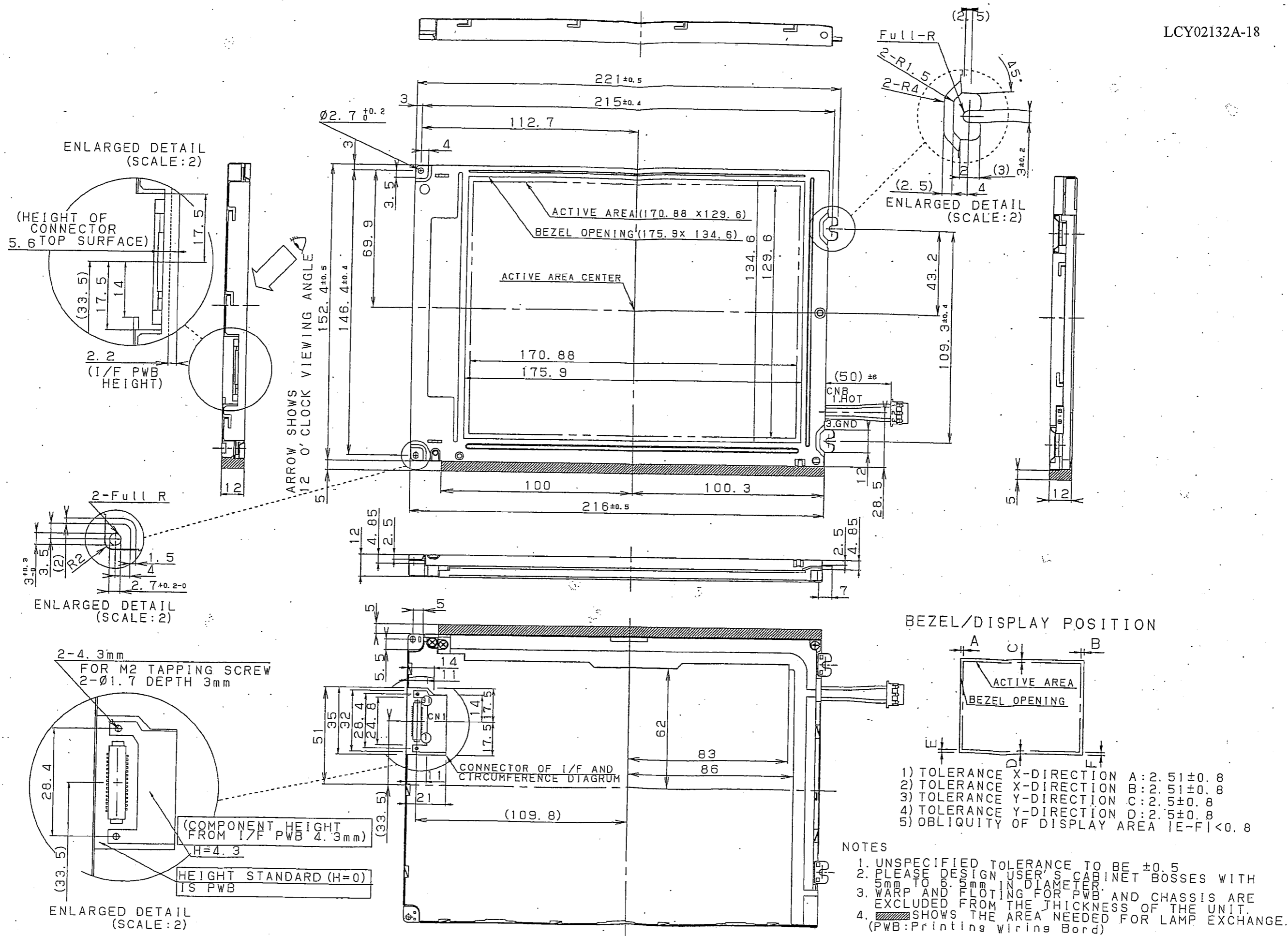
FIG1. LQ084V1DG21 OUTLINE DEMENSIONS
